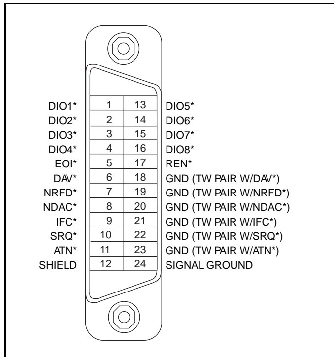
Figure B-1. GPIB Connector
